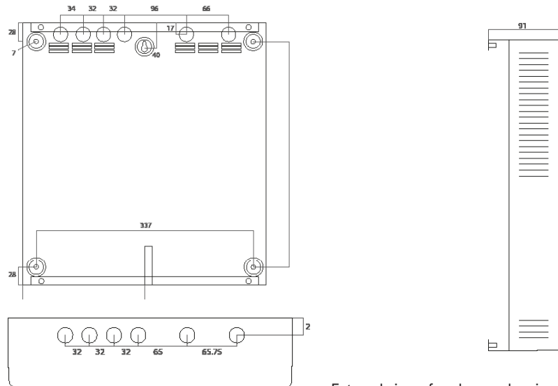
External view of enclosure showing mounting holes
