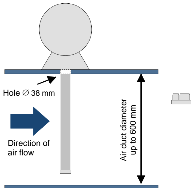
Fig. 12: Venturi tubes up to 600 mm
